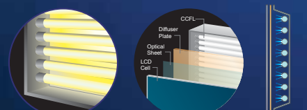
CCFL (Cold Cathode Fluorescent Lamp) Conventional CCFL Backlight
