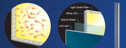
White LED (Light Emitting Diode) Edge-type White LED
